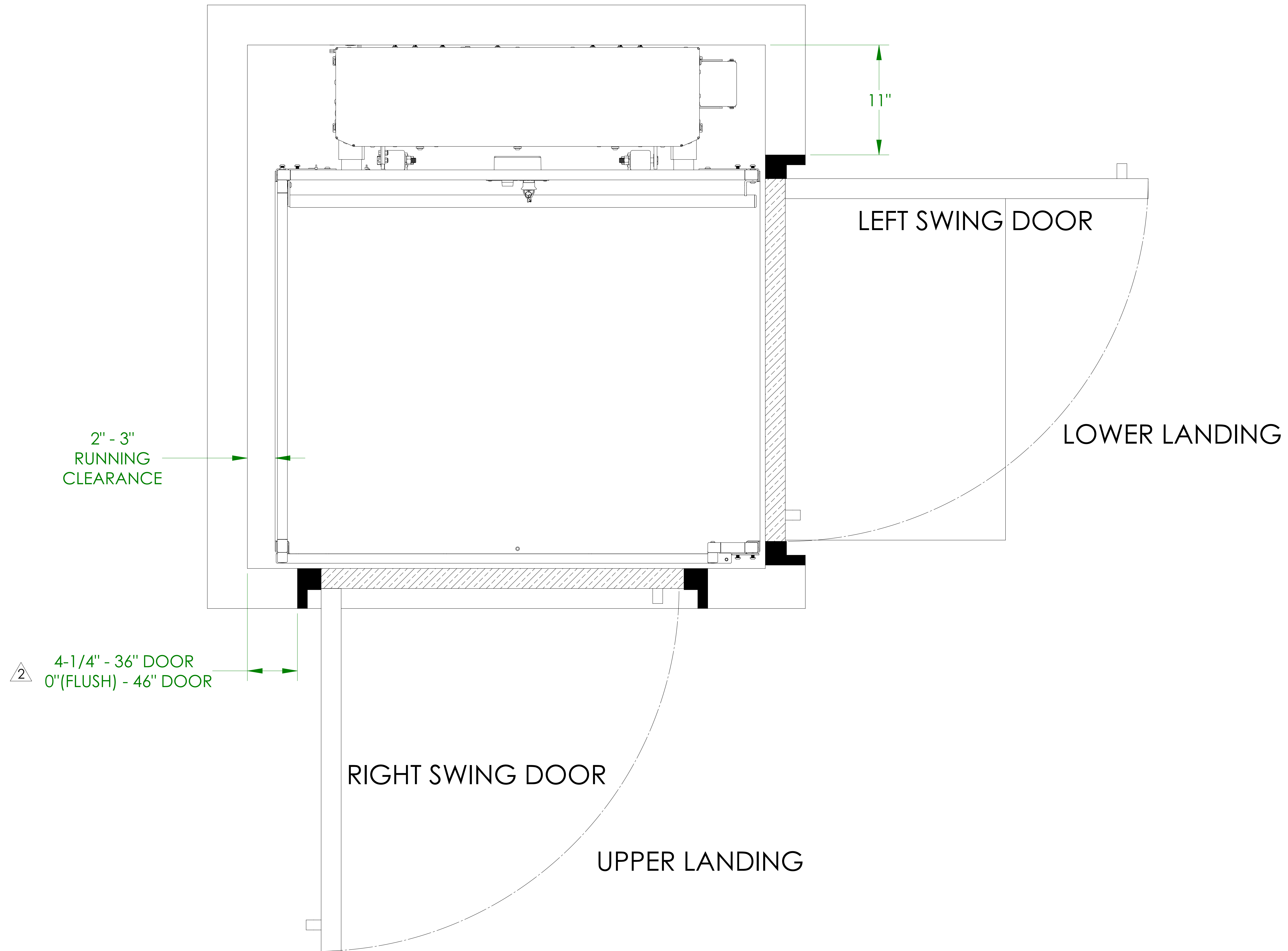
PLAN VIEW (RIGHT HAND UNIT SHOWN)
