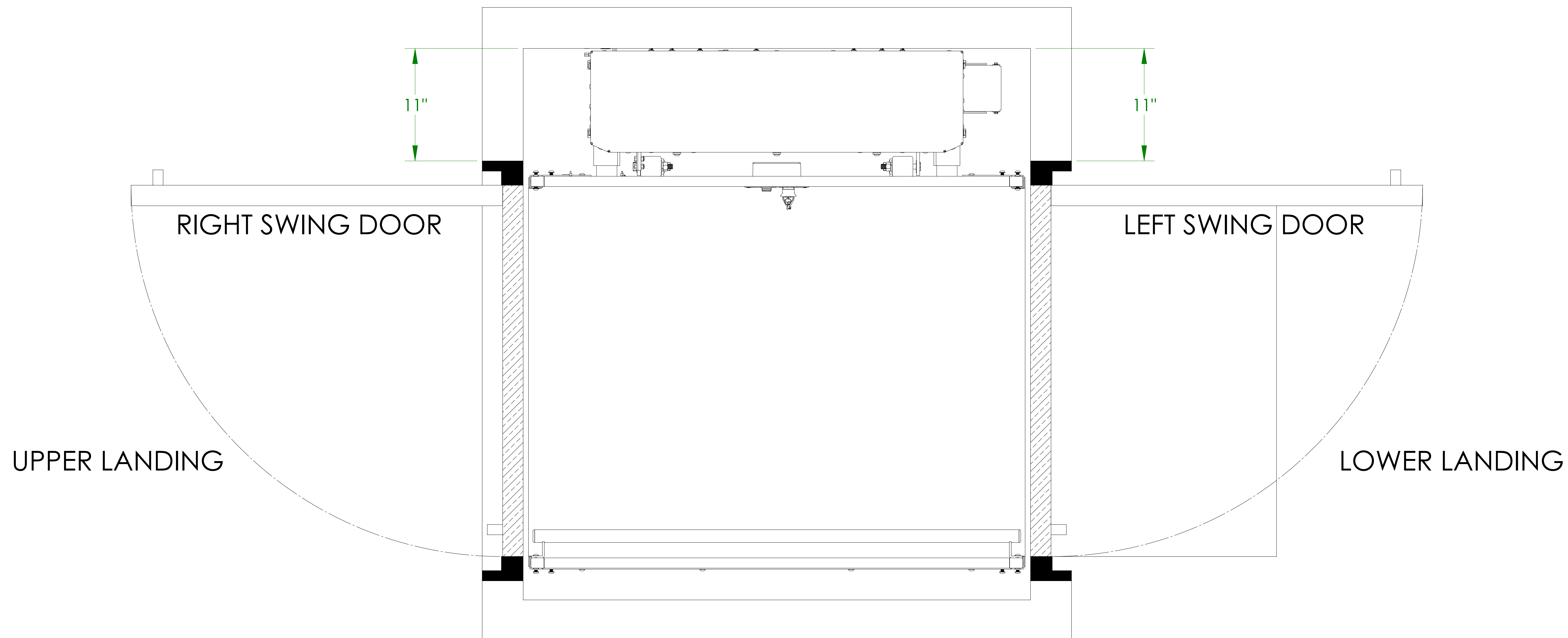
PLAN VIEW (RIGHT HAND UNIT SHOWN)
